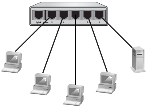
Figure 4 Single AT-FS705LE Switch Topology
